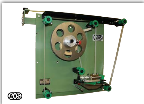
Tape coater without drying stretch
