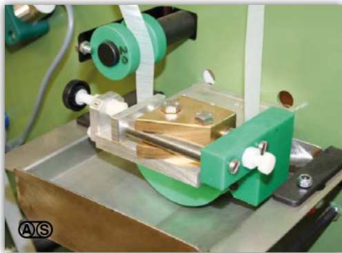
Tape coater with adhesive container
